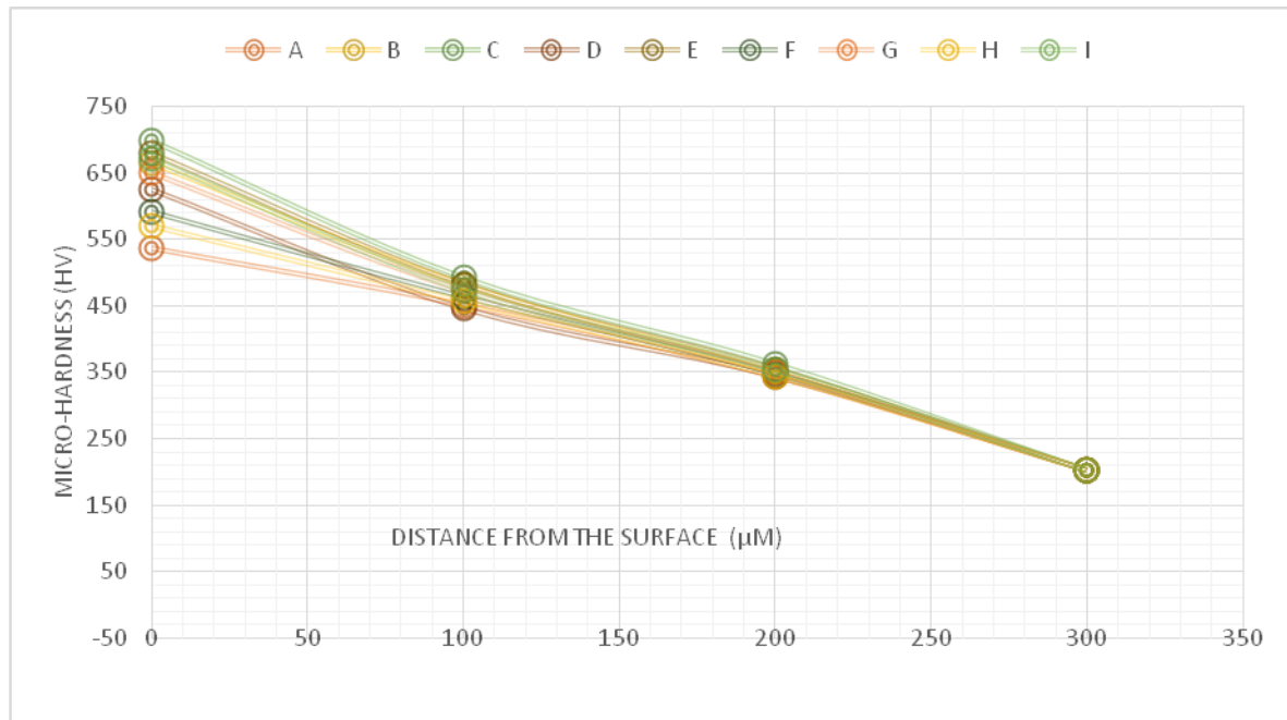
Fig. 4 micro-hardness results
